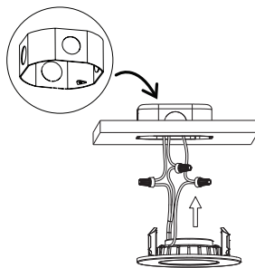
J-box Installation
