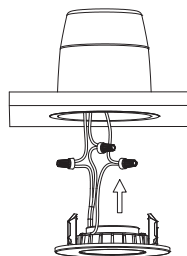
Can Installation
