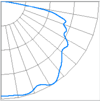
SCS/PS60/8xx/UD/G (Typical performance @4000K with Garage distribution)*
