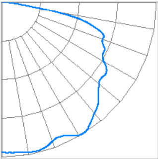
SCS/70W/8xx/UD/G (Typical performance @4000K with Garage distribution)*
