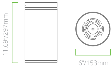
6" SURFACE MOUNT (CSMWP61)
