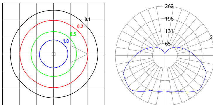
VTU-20/20W/830-U-xx (Wall Mount)
