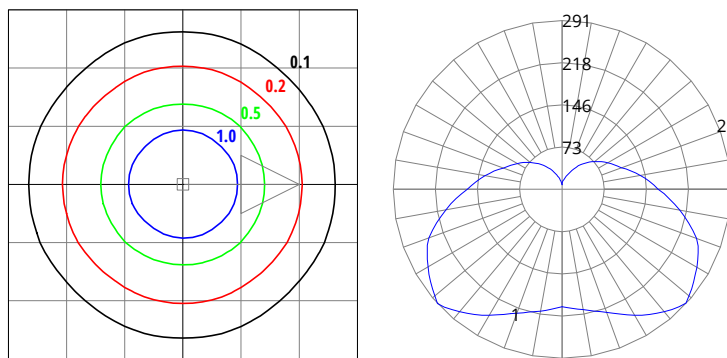
VTU-20/20W/850-U-xx (Wall Mount)
