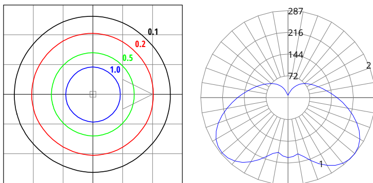
VTU-20/20W/850-U-xx (Ceiling Mount)
