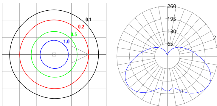
VTU-20/20W/830-U-xx (Ceiling Mount)
