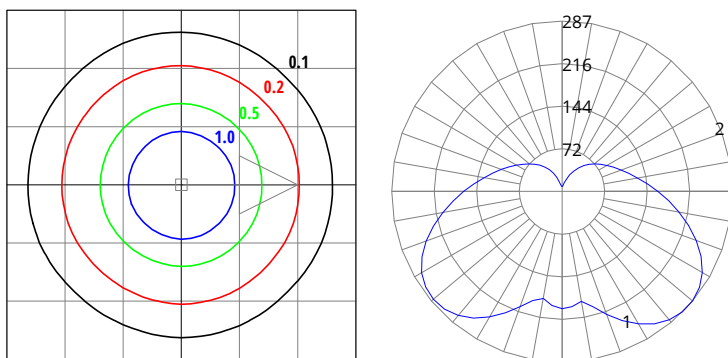
VTU-20/20W/840-U-xx (Ceiling Mount)
