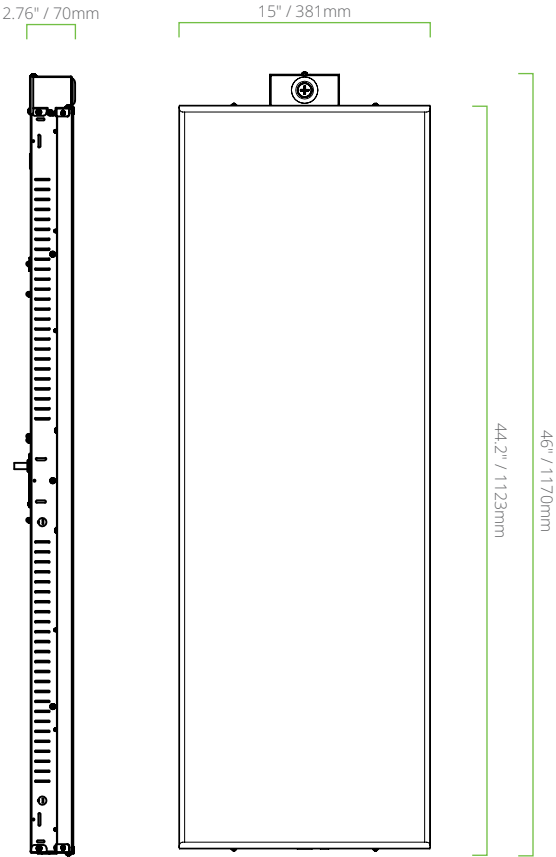
MODELS: LHS1-PS440W 440W Weight: 16.2 lbs / 7.37 kg Master Carton Weight: 10.24 lbs Dimensions: 47.05" x 4.13" x 15.94"
