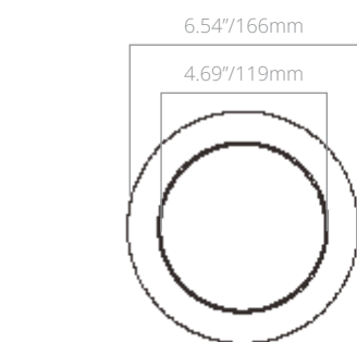
6" Trim Ring
