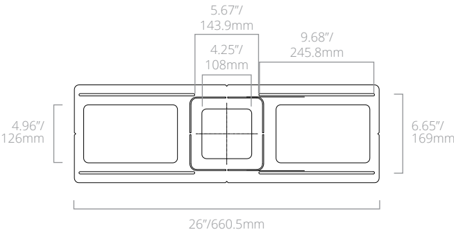
RIP-46S Rough-In Plate for Square Downlights
