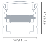
Series 400 with lens
