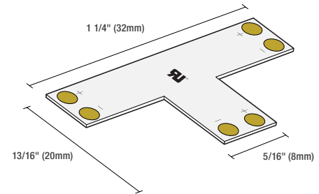
67631 - T SHAPE PCB JOINER
