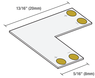
67630 - L SHAPE PCB JOINER
