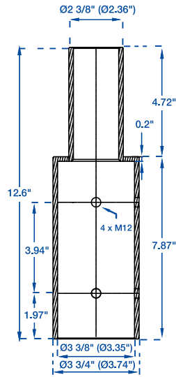
3" to 2 3/8" PA-TA-R3-BK PA-TA-R3-BZ
