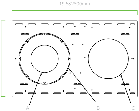
DL-NCPSJ NEW CONSTRUCTION PLATE STUD/JOIST
