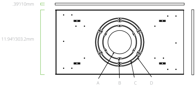
DL-NCPTG NEW CONSTRUCTION PLATE T-GRID
