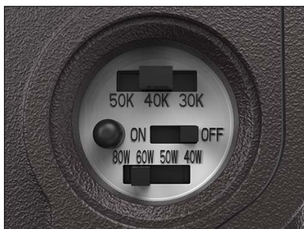
Power, CCT, and Photocell Selector Switches
