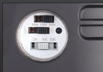
Power, CCT, & Photocell Selector Switches
